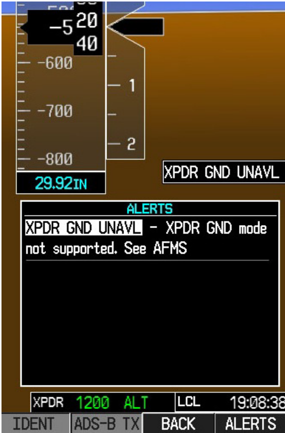
Figure 1-3 XPDR GND UNAVL Annunciation Display
