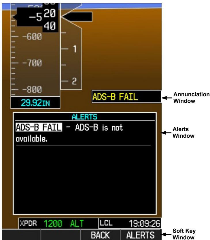
Figure 1-2 Annunciation Display
